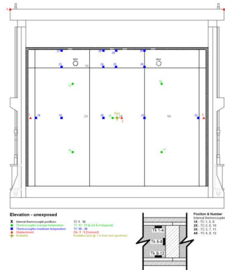
Figure B.1: Thermocam drawing
