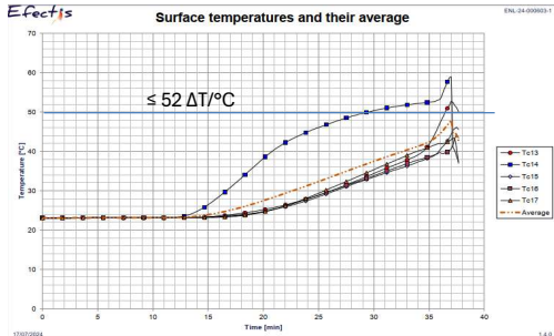
Figure B.2: Surface temperatures and their average
