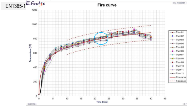
Figure A.1: Furnace temperature
