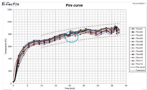
Figure A.1: Furnace temperature
